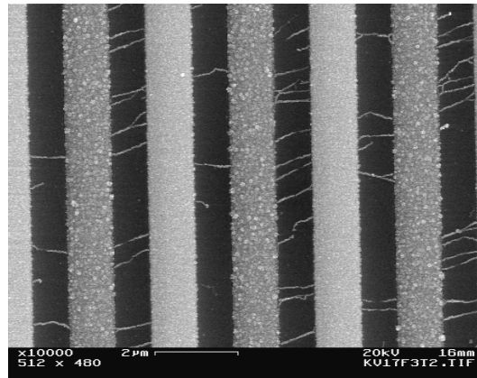
Electron microscope image of metalized DNA Bridges/Wires
